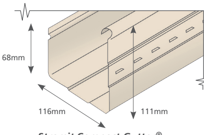
Stramit Compact Gutter® Slotted
