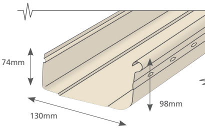
Stramit Queenslander Quad® Slotted Hi-Front
