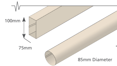
Stramit® Downpipes
